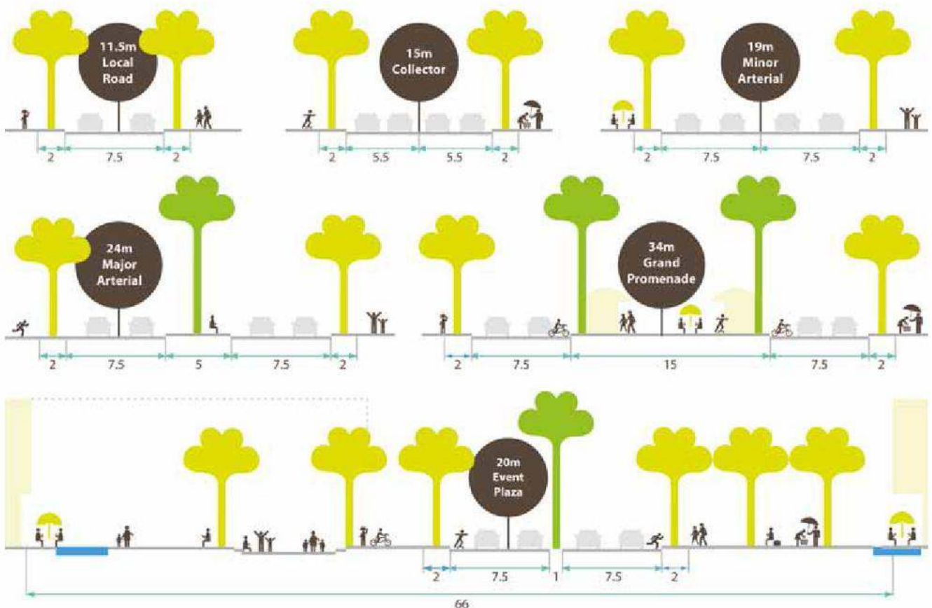
Traffic Plan & Street Sections
