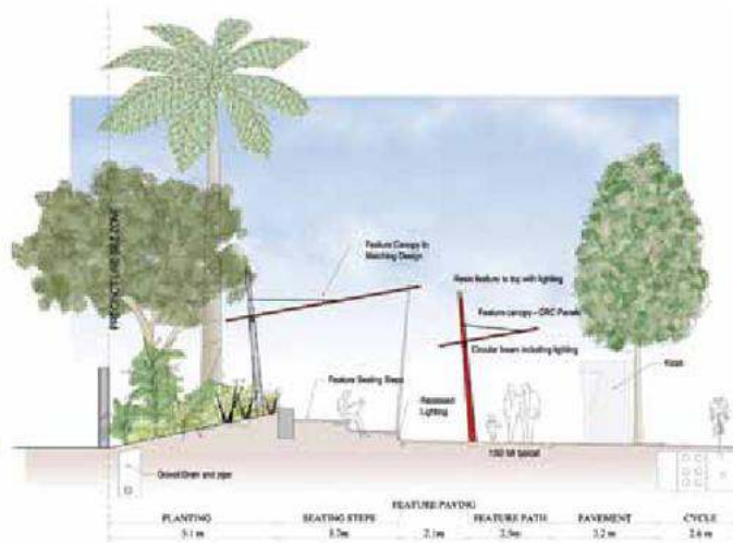
Sectional Drawings of Linear Park
