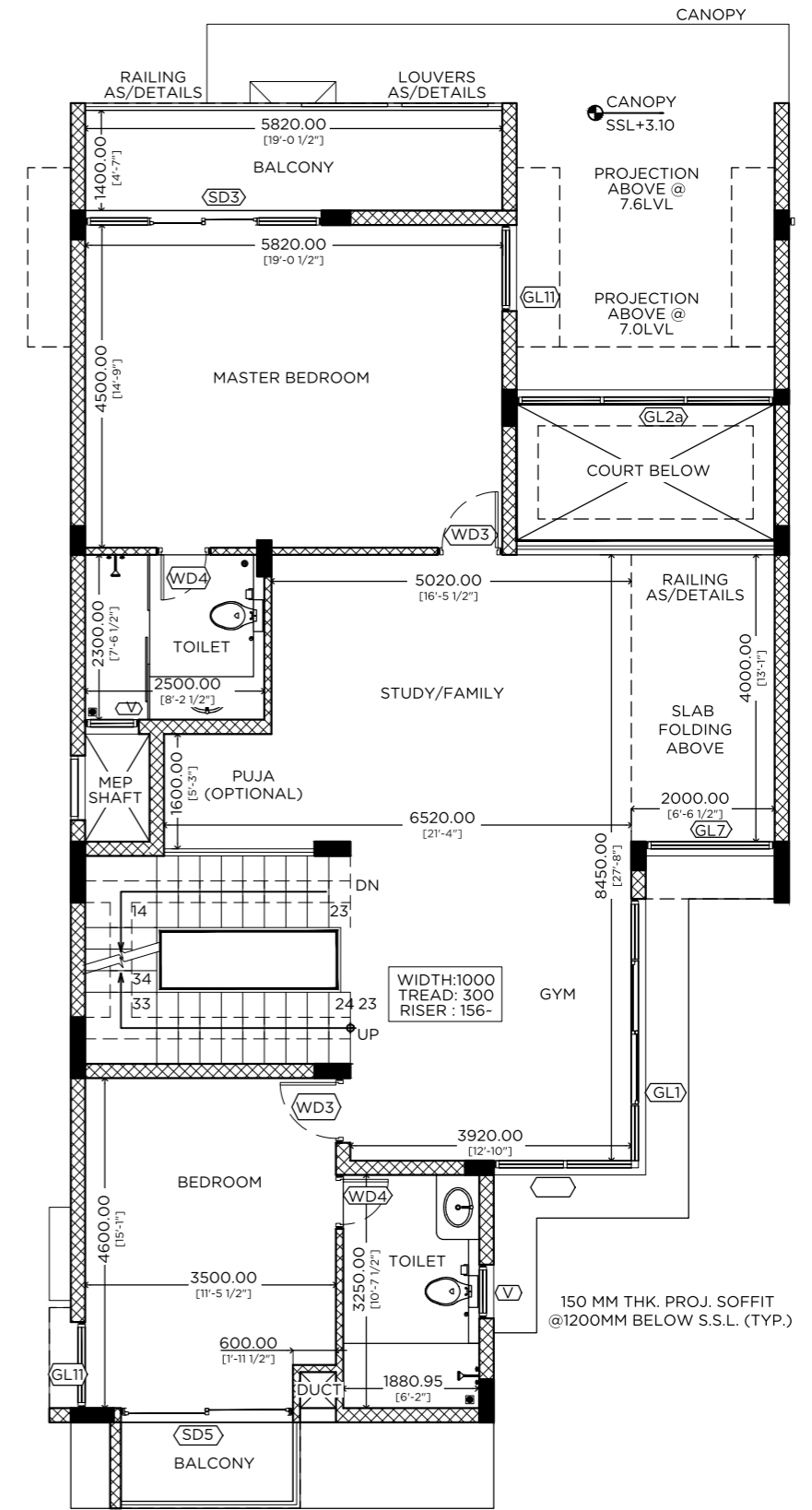
FIRST FLOOR
